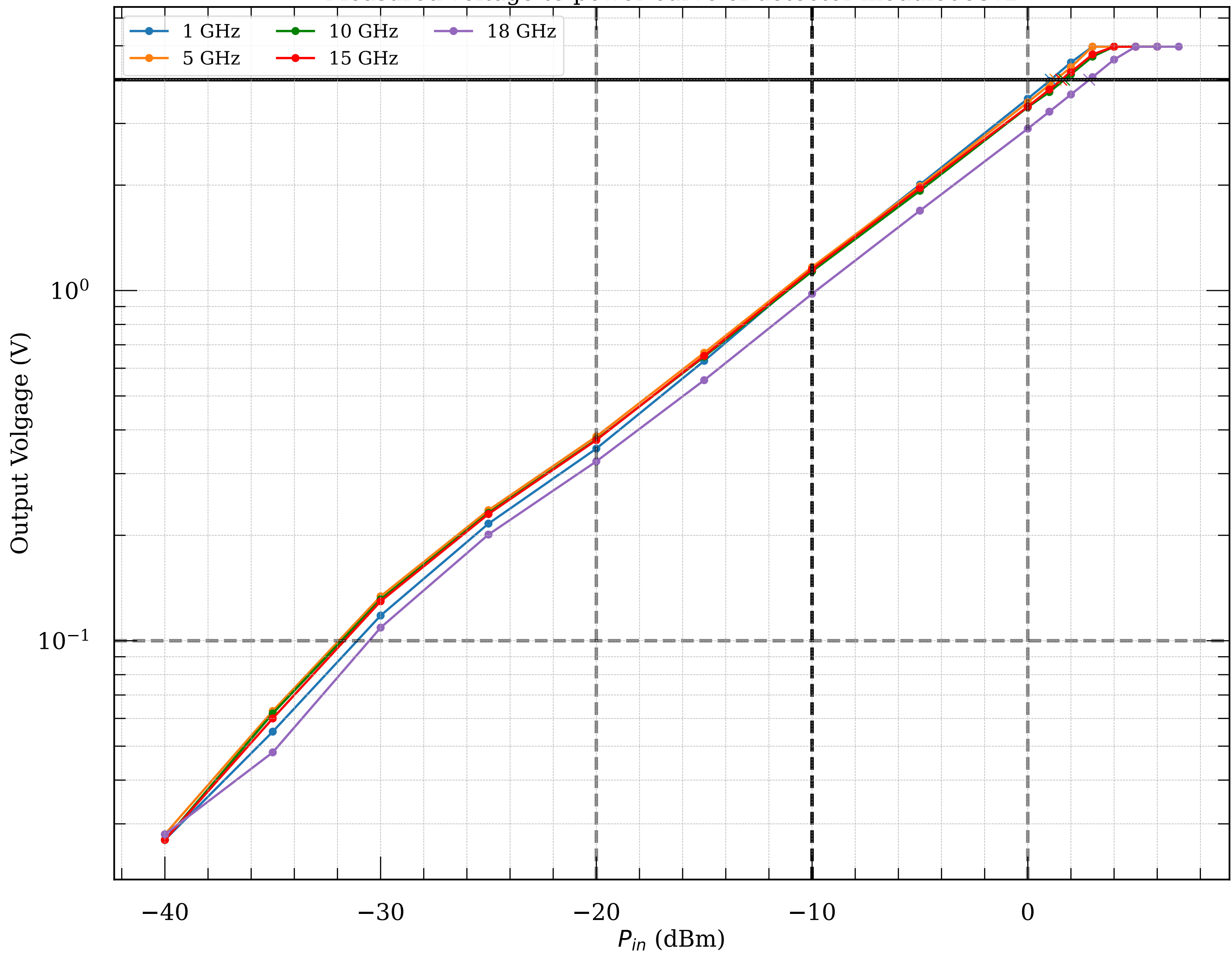
Measured voltage-to-power curve of detector module068v2
